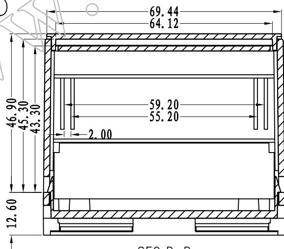
SEC B-B
