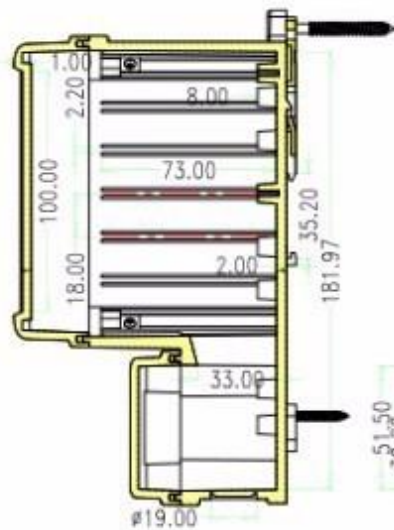
SEC C-C
