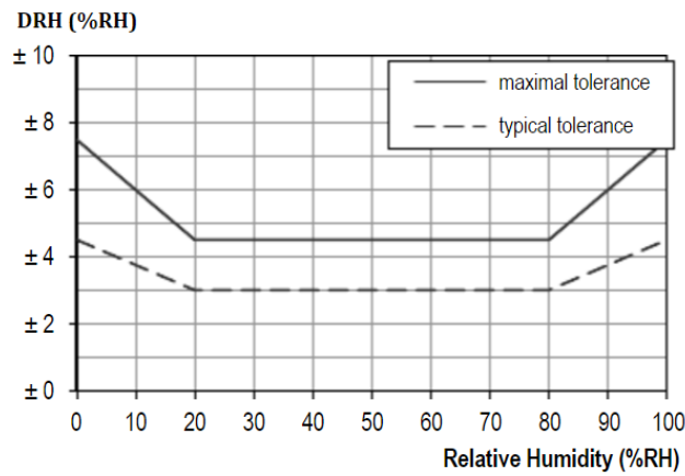
Figure3 Humidity measurement accuracy under different humidity conditions
